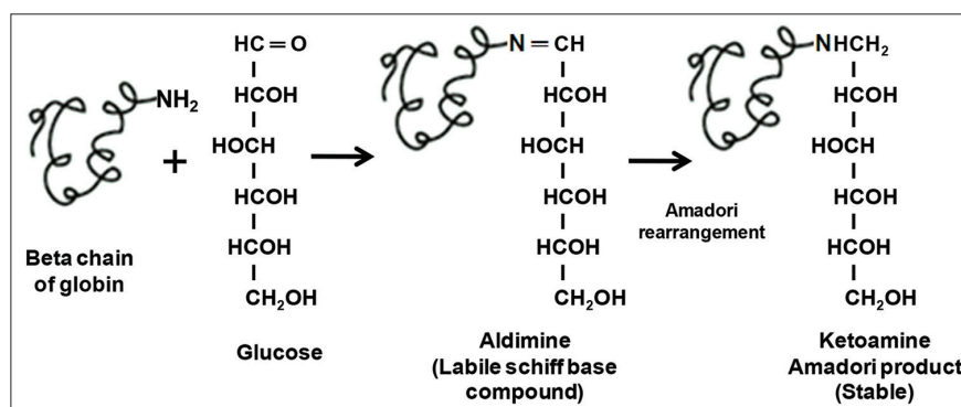
Figure 1: Mechanism of non-enzymatic glycosylation of hemoglobin.
